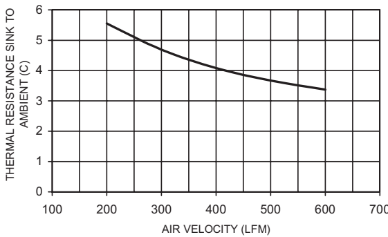
613 THERMAL PERFORMANCE
