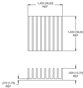
MECHANICAL DIMENSIONS
