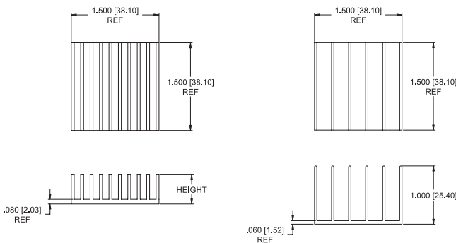
MECHANICAL DIMENSIONS
