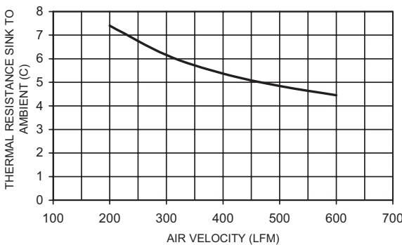
615 THERMAL PERFORMANCE
