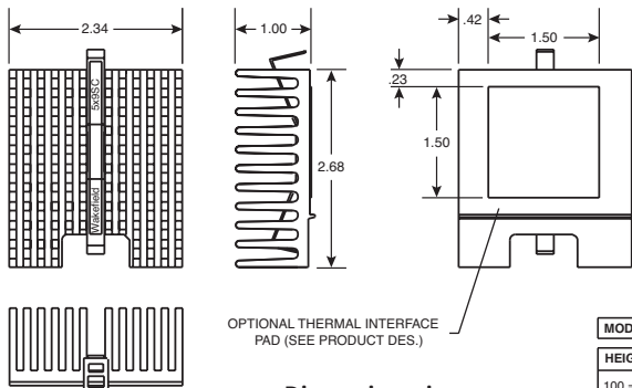
Dimensions: in.
