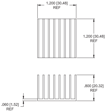
MECHANICAL DIMENSIONS
