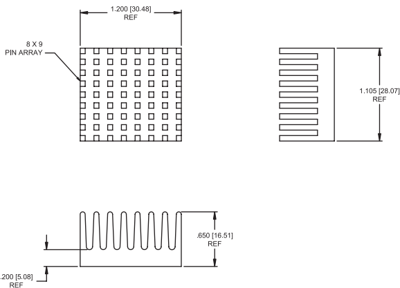
MECHANICAL DIMENSIONS
