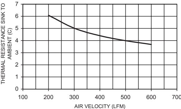
611 THERMAL PERFORMANCE
