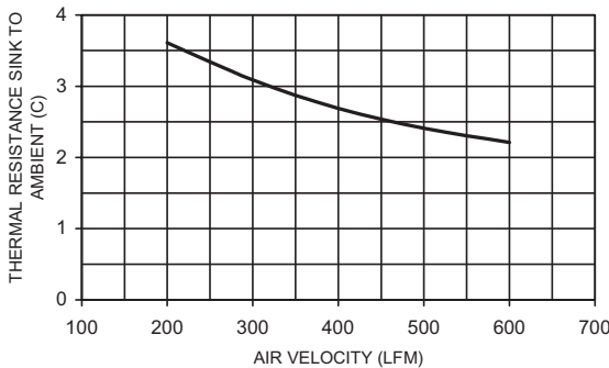
612 THERMAL PERFORMANCE
