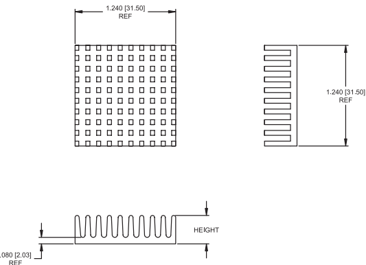
MECHANICAL DIMENSIONS
