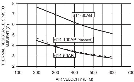
614 THERMAL PERFORMANCE
